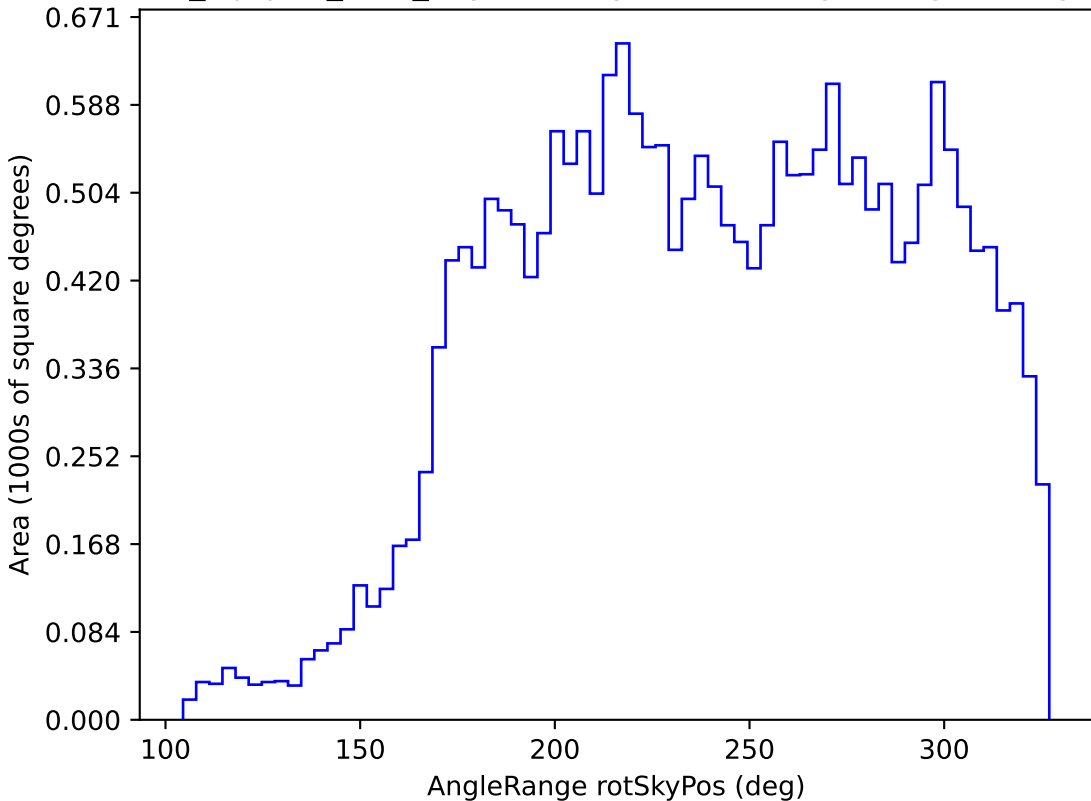
noroll_mjdp60_v3.4_10yrs All sky u band: AngleRange rotSkyPos
