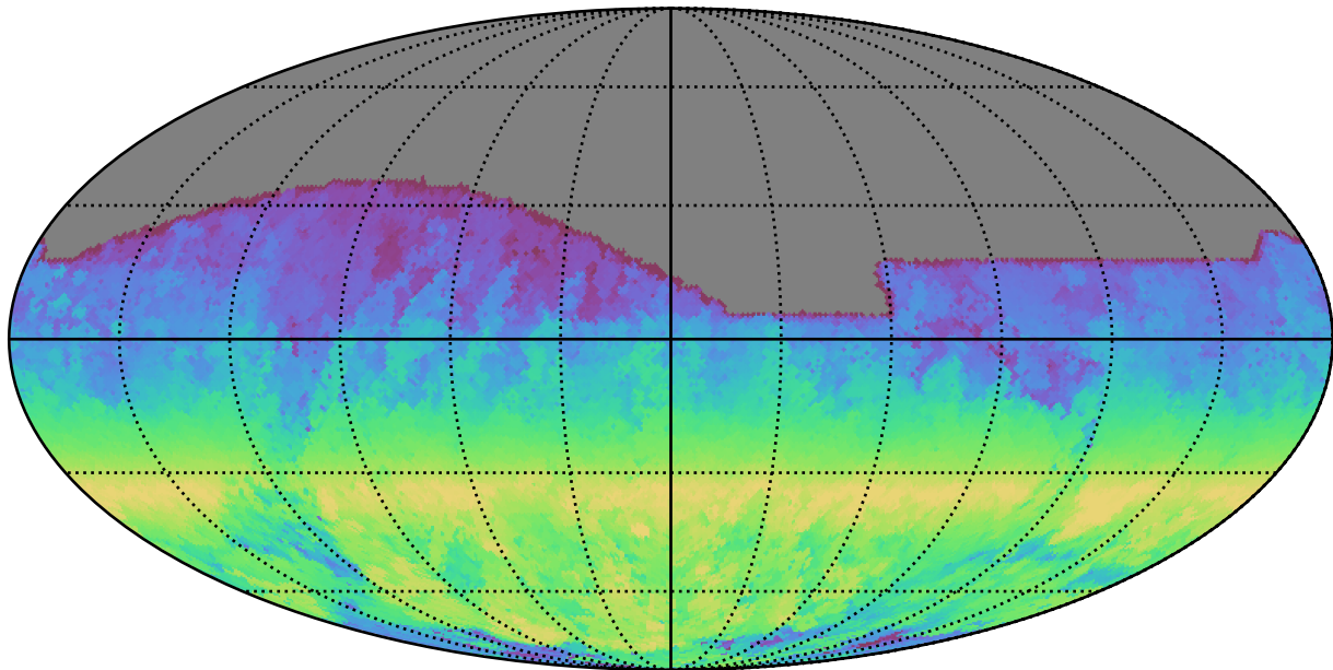
noroll_mjdp60_v3.4_10yrs All sky r band: AngleRange rotSkyPos
