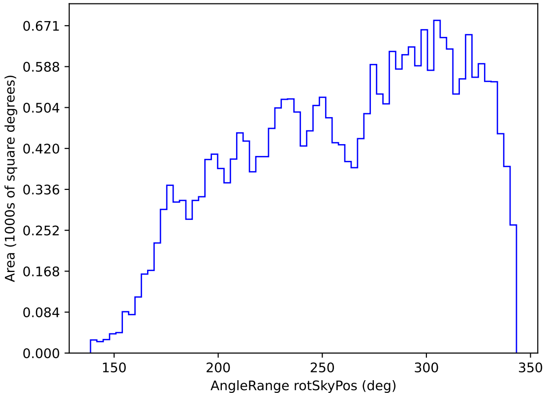
noroll_mjdp60_v3.4_10yrs All sky i band: AngleRange rotSkyPos
