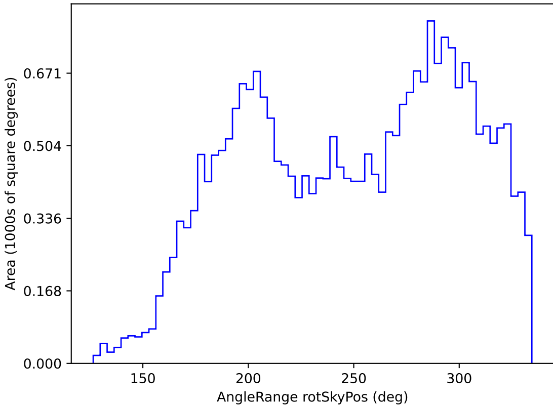
noroll_mjdp60_v3.4_10yrs All sky g band: AngleRange rotSkyPos
