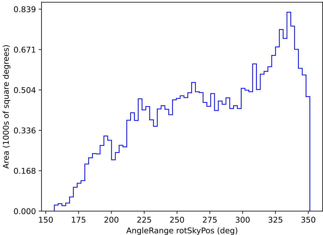
noroll_mjdp60_v3.4_10yrs All sky all bands: AngleRange rotSkyPos
