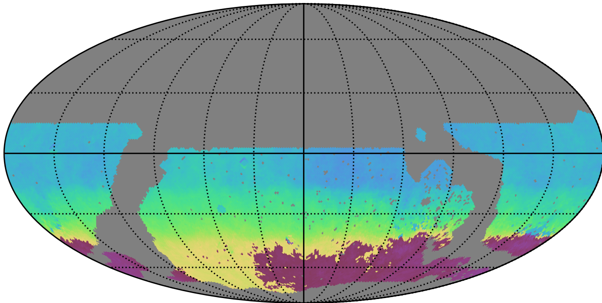
noroll_mjdp60_v3.4_10yrs WFD z band: AngleMean rotSkyPos
