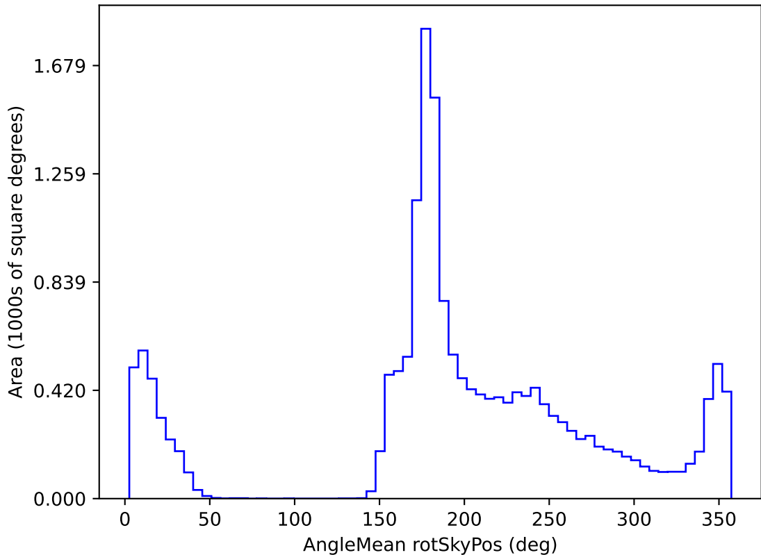
noroll_mjdp60_v3.4_10yrs WFD z band: AngleMean rotSkyPos
