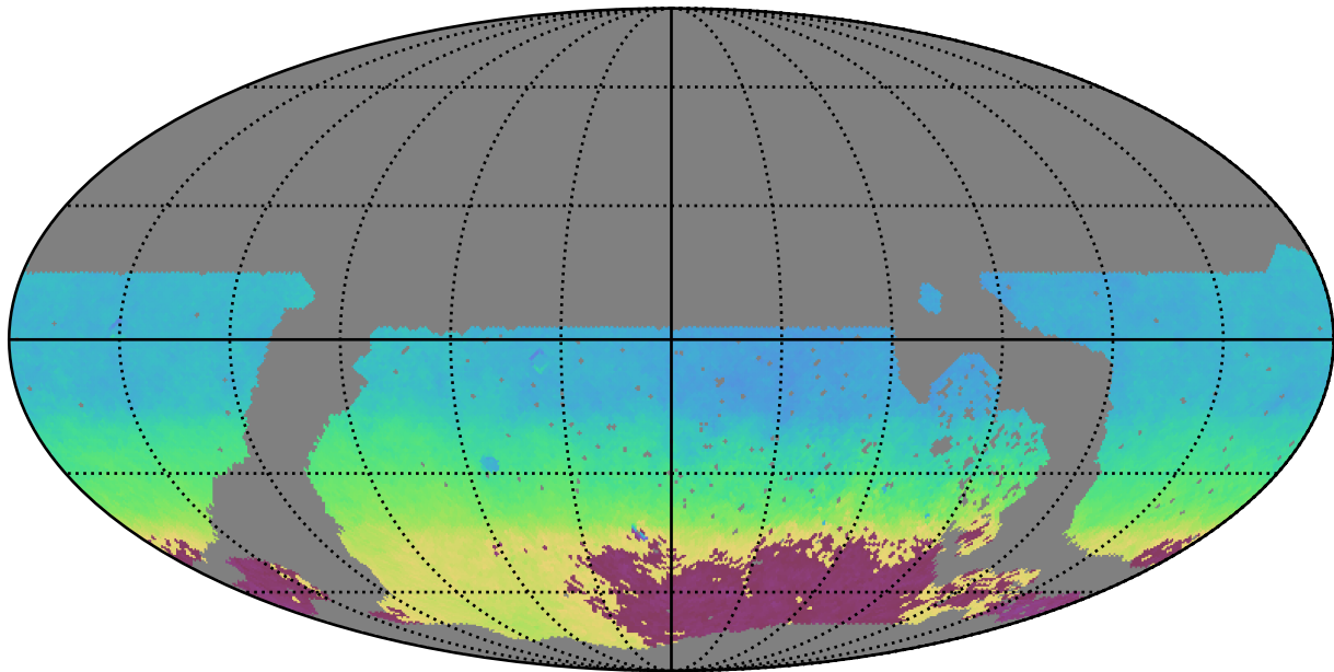
noroll_mjdp60_v3.4_10yrs WFD y band: AngleMean rotSkyPos
