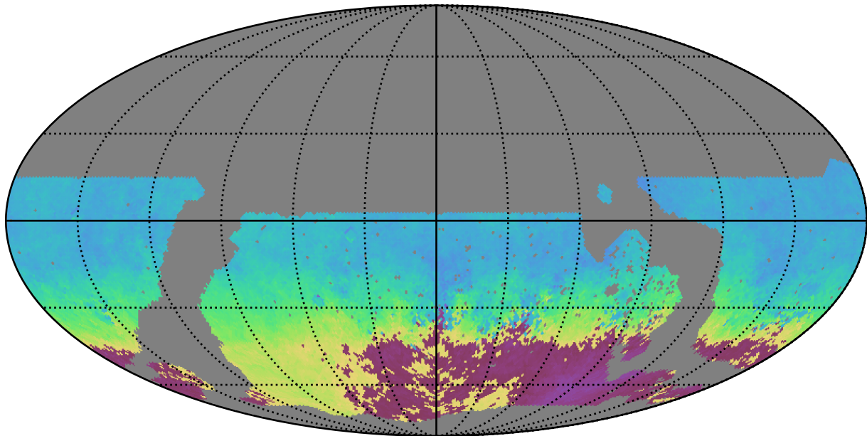
noroll_mjdp60_v3.4_10yrs WFD u band: AngleMean rotSkyPos
