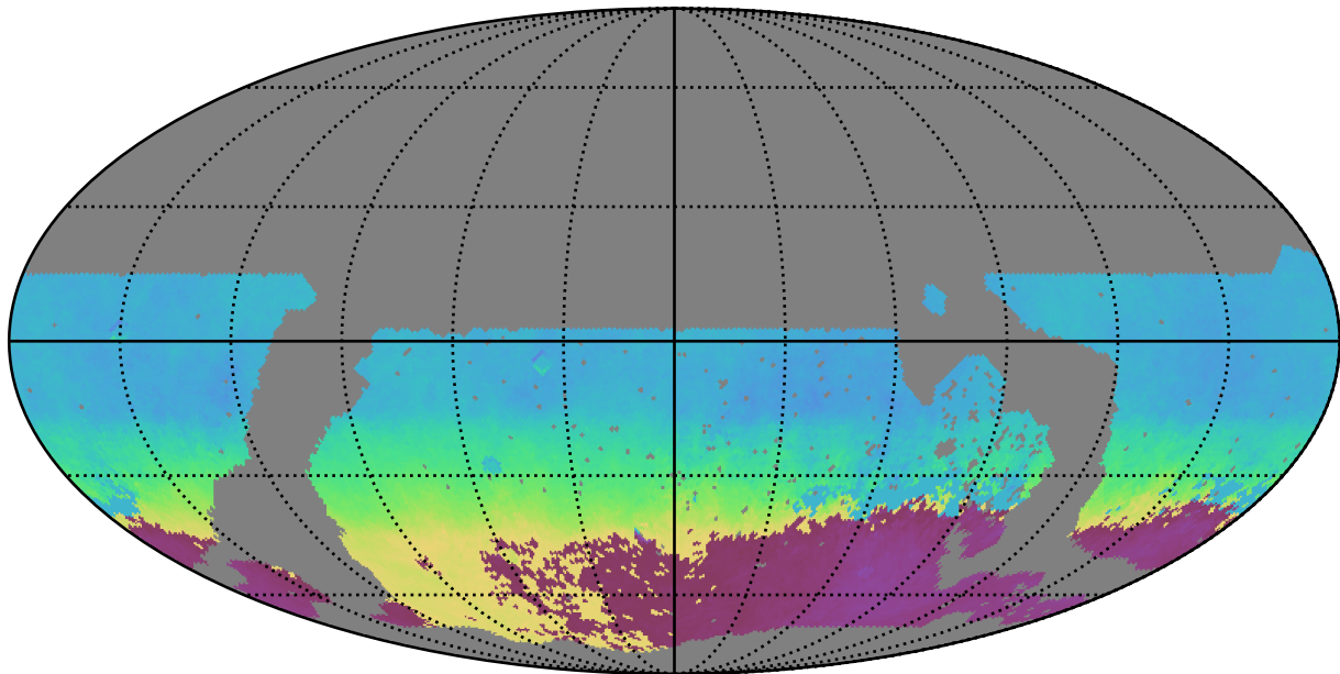
noroll_mjdp60_v3.4_10yrs WFD r band: AngleMean rotSkyPos
