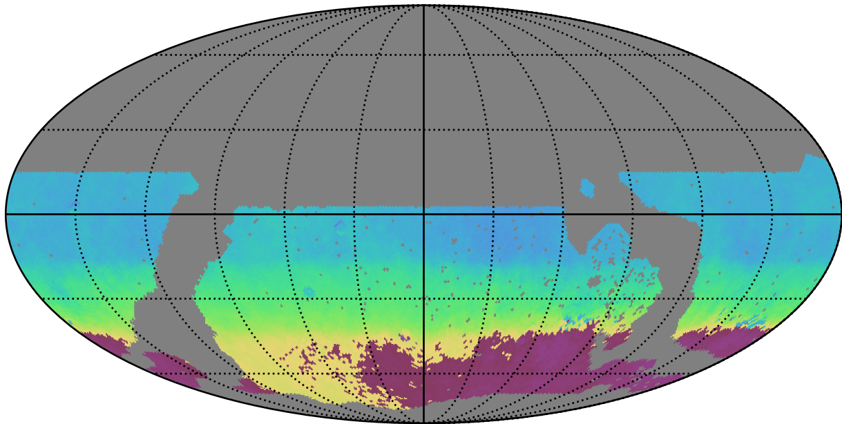
noroll_mjdp60_v3.4_10yrs WFD i band: AngleMean rotSkyPos
