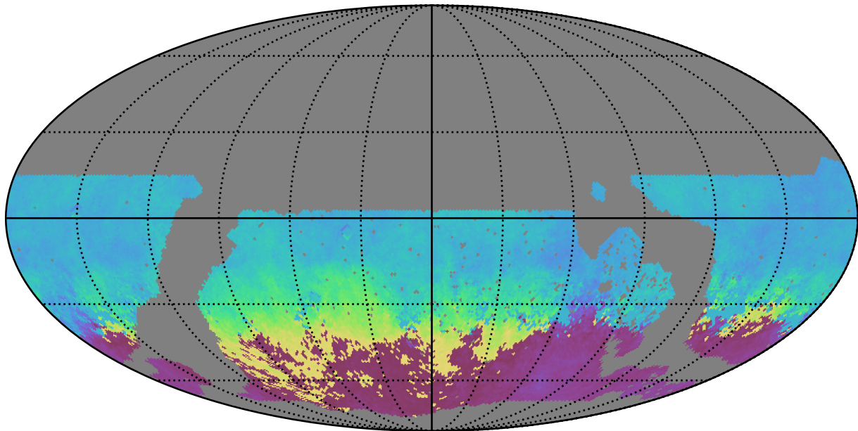
noroll_mjdp60_v3.4_10yrs WFD g band: AngleMean rotSkyPos
