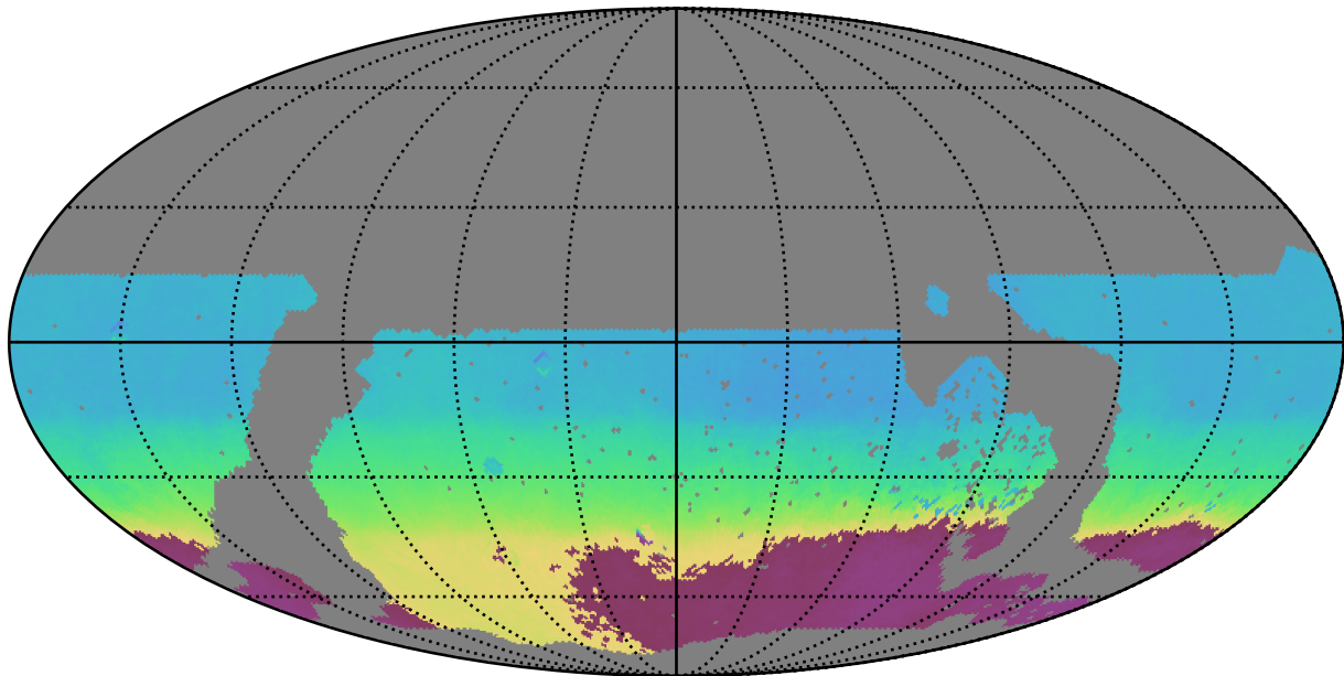
noroll_mjdp60_v3.4_10yrs WFD all bands: AngleMean rotSkyPos
