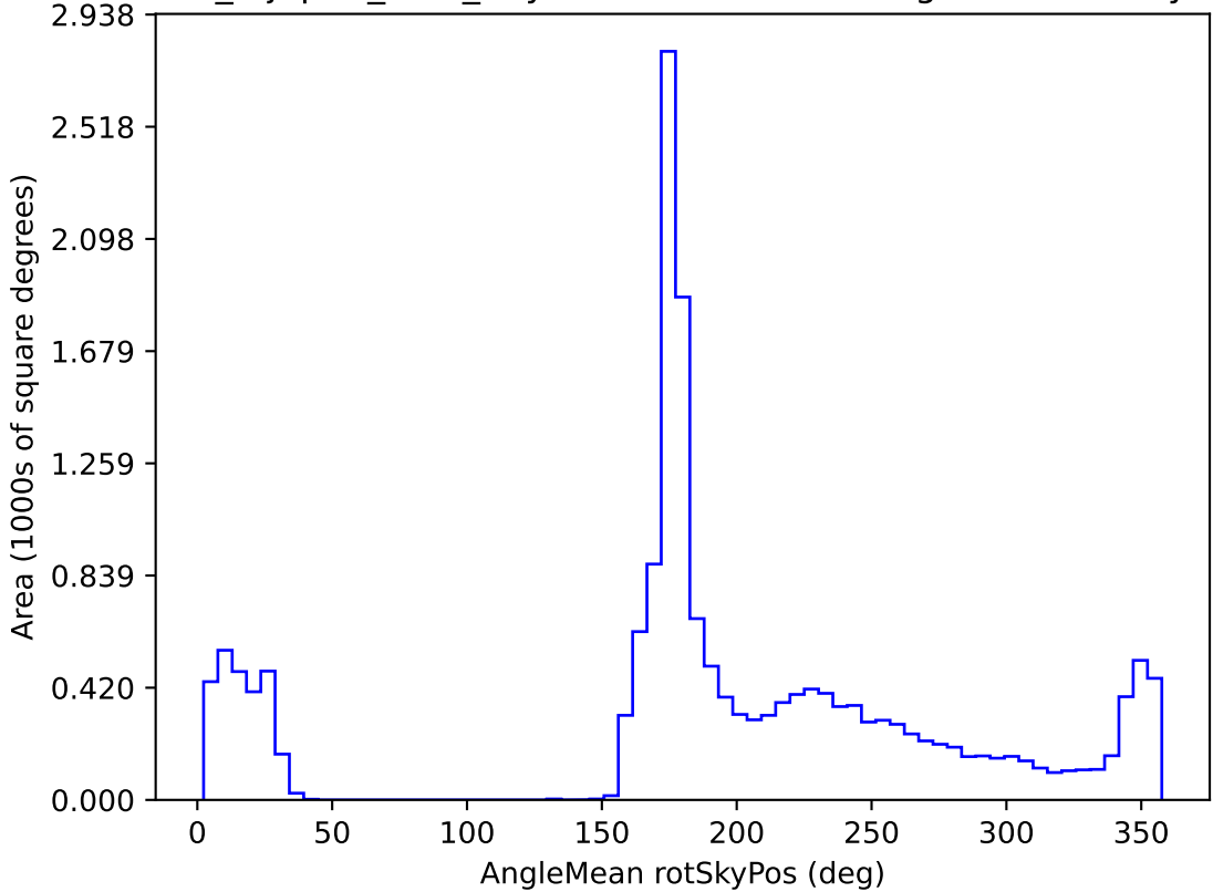
noroll_mjdp60_v3.4_10yrs WFD all bands: AngleMean rotSkyPos
