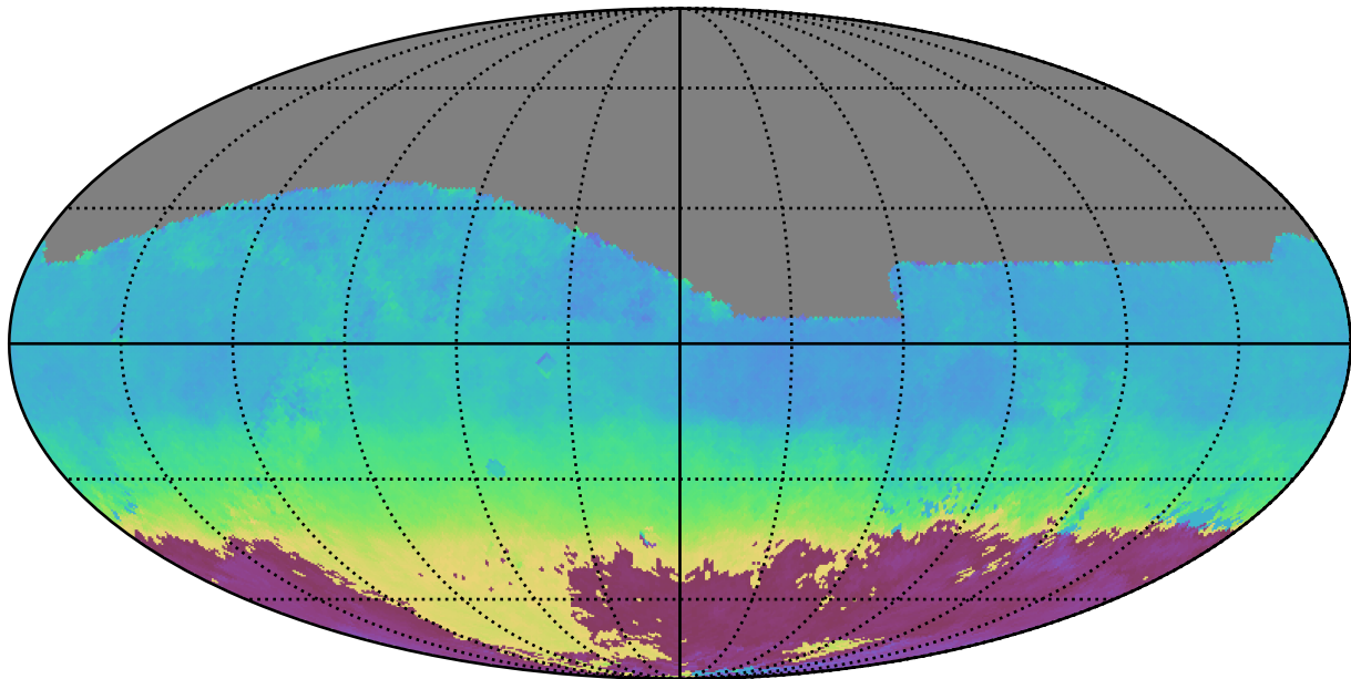
noroll_mjdp60_v3.4_10yrs All sky z band: AngleMean rotSkyPos
