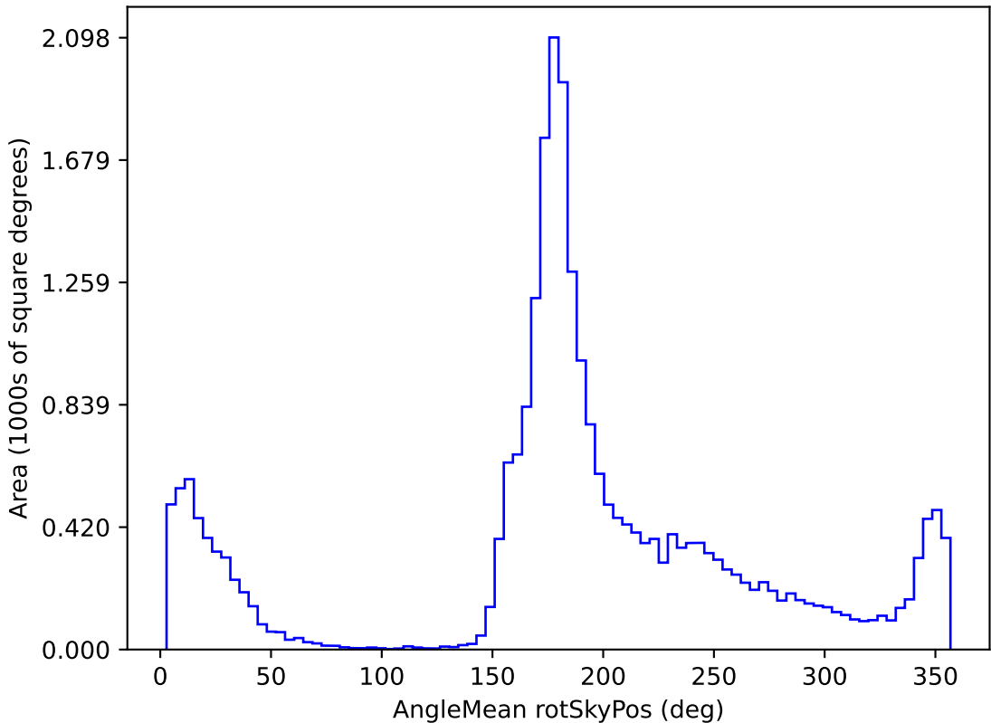
noroll_mjdp60_v3.4_10yrs All sky z band: AngleMean rotSkyPos
