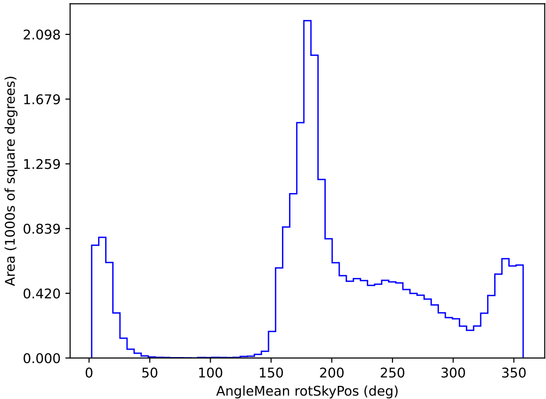
noroll_mjdp60_v3.4_10yrs All sky y band: AngleMean rotSkyPos
