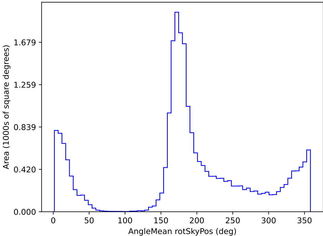
noroll_mjdp60_v3.4_10yrs All sky u band: AngleMean rotSkyPos
