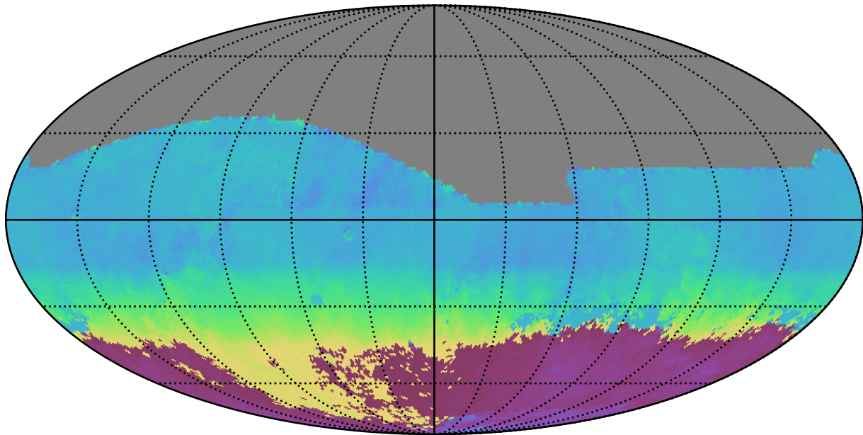
noroll_mjdp60_v3.4_10yrs All sky r band: AngleMean rotSkyPos
