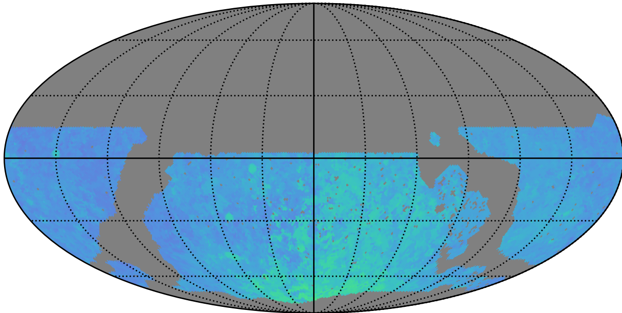
noroll_mjdp60_v3.4_10yrs WFD z band: 80thPercentile Season Length
