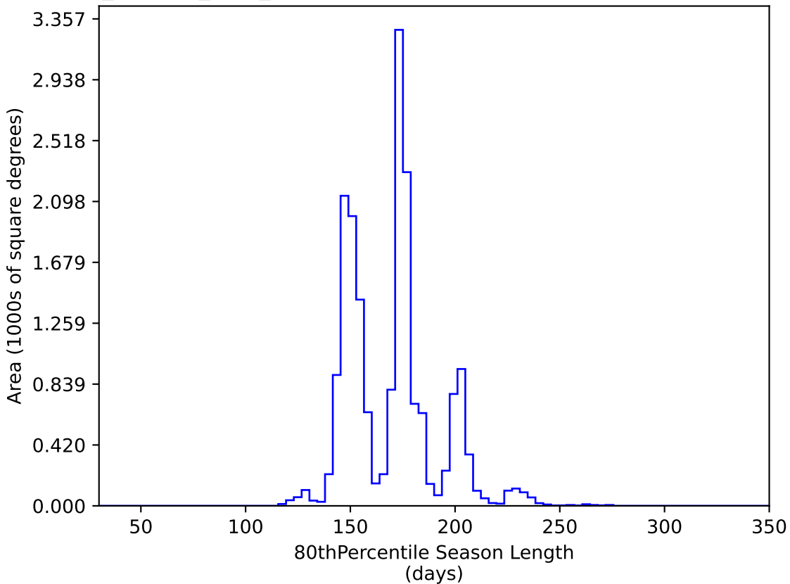
noroll_mjdp60_v3.4_10yrs WFD y band: 80thPercentile Season Length
