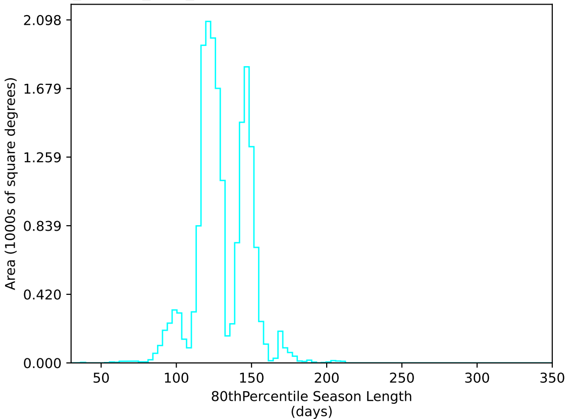
noroll_mjdp60_v3.4_10yrs WFD u band: 80thPercentile Season Length
