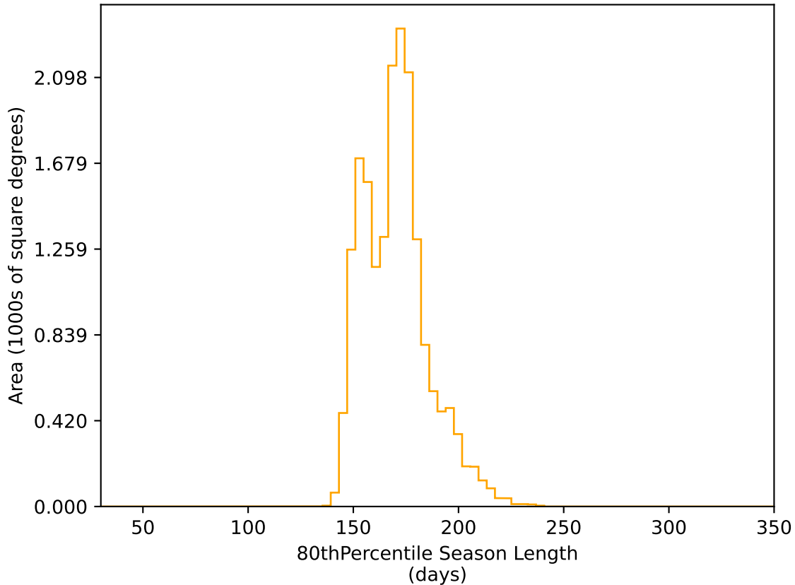
noroll_mjdp60_v3.4_10yrs WFD r band: 80thPercentile Season Length
