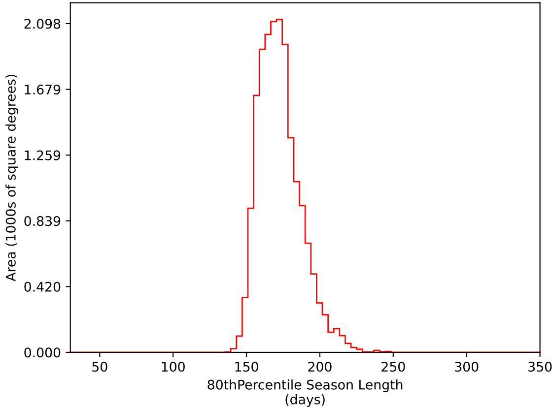
noroll_mjdp60_v3.4_10yrs WFD i band: 80thPercentile Season Length
