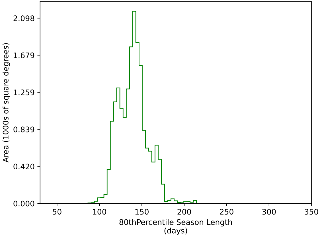
noroll_mjdp60_v3.4_10yrs WFD g band: 80thPercentile Season Length
