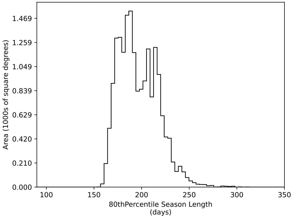
noroll_mjdp60_v3.4_10yrs WFD all bands: 80thPercentile Season Length
