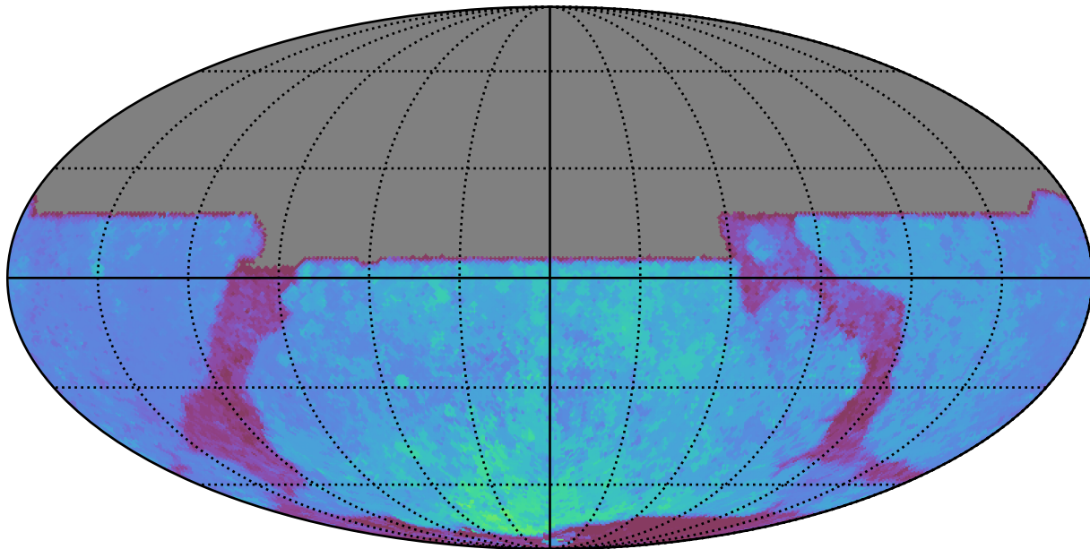
noroll_mjdp60_v3.4_10yrs All sky y band: 80thPercentile Season Length
