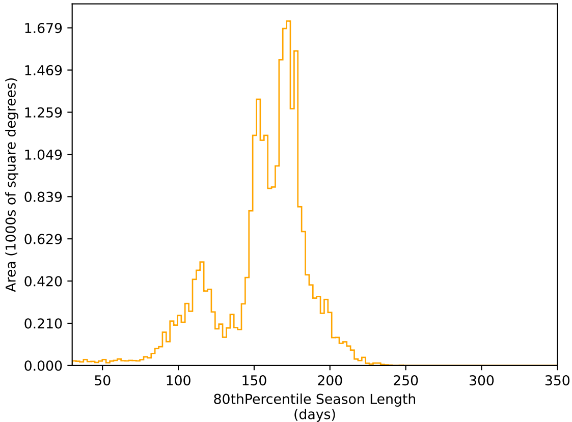
noroll_mjdp60_v3.4_10yrs All sky r band: 80thPercentile Season Length
