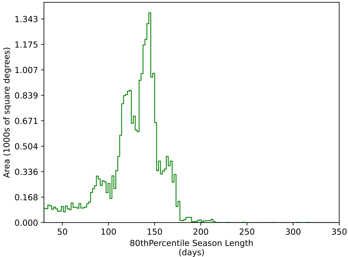
noroll_mjdp60_v3.4_10yrs All sky g band: 80thPercentile Season Length
