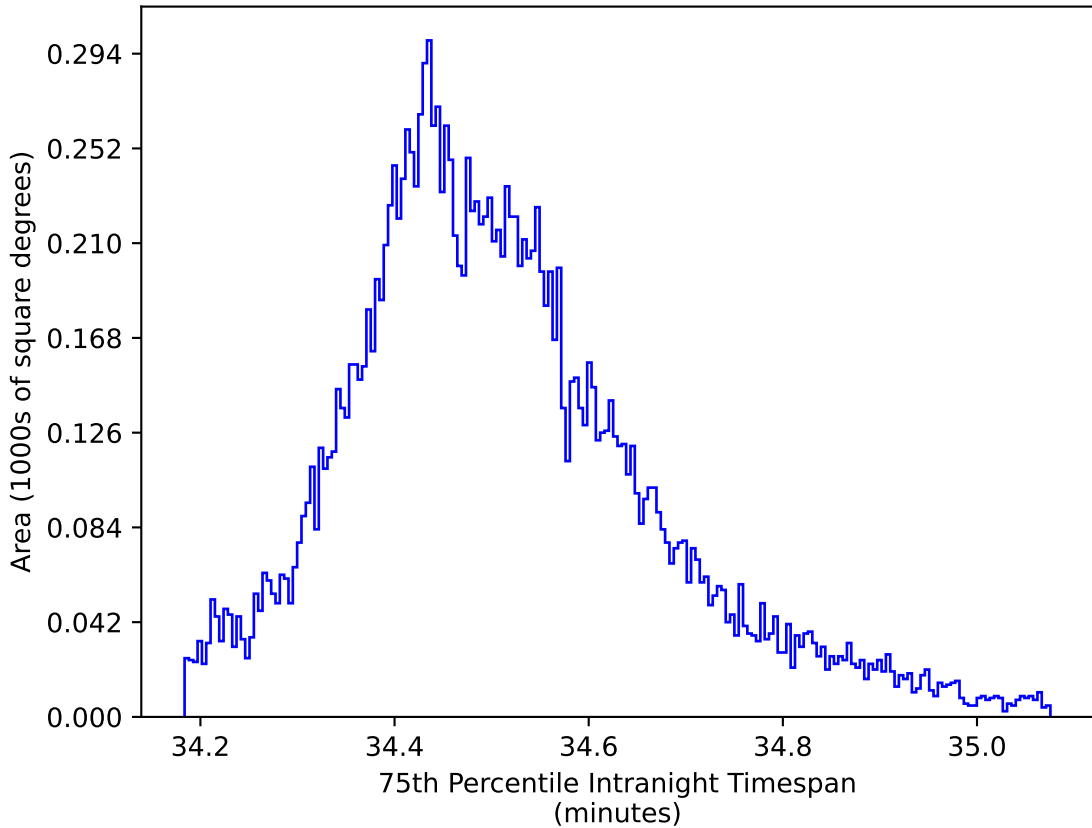
noroll_mjdp60_v3.4_10yrs WFD zy bands: 75th Percentile Intranight Timespan
