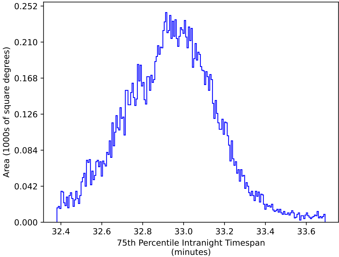
noroll_mjdp60_v3.4_10yrs WFD y band: 75th Percentile Intranight Timespan
