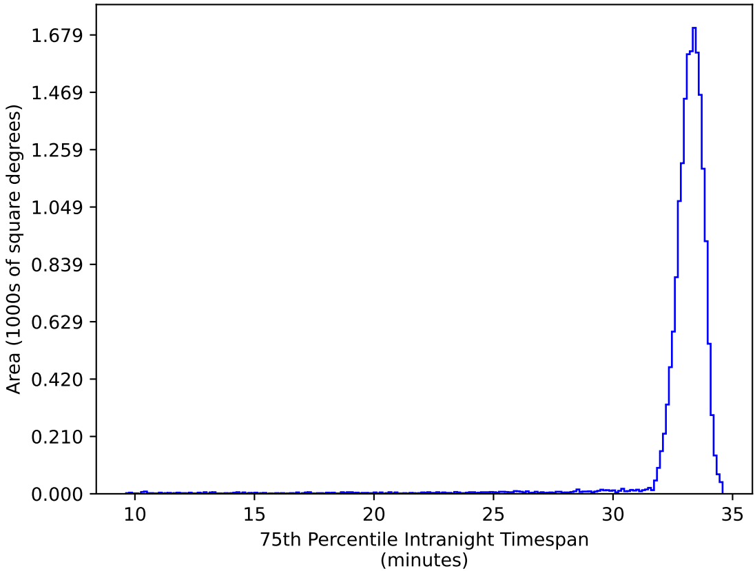
noroll_mjdp60_v3.4_10yrs WFD ug bands: 75th Percentile Intranight Timespan
