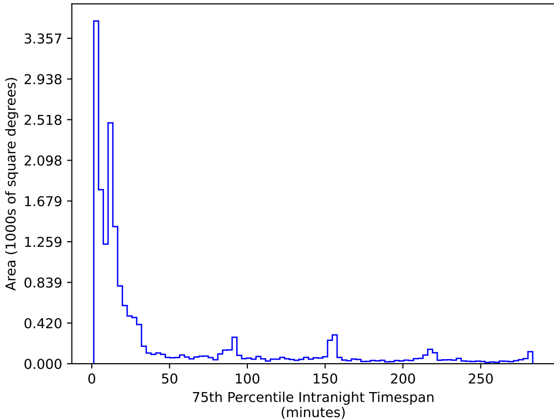
noroll_mjdp60_v3.4_10yrs WFD r band: 75th Percentile Intranight Timespan
