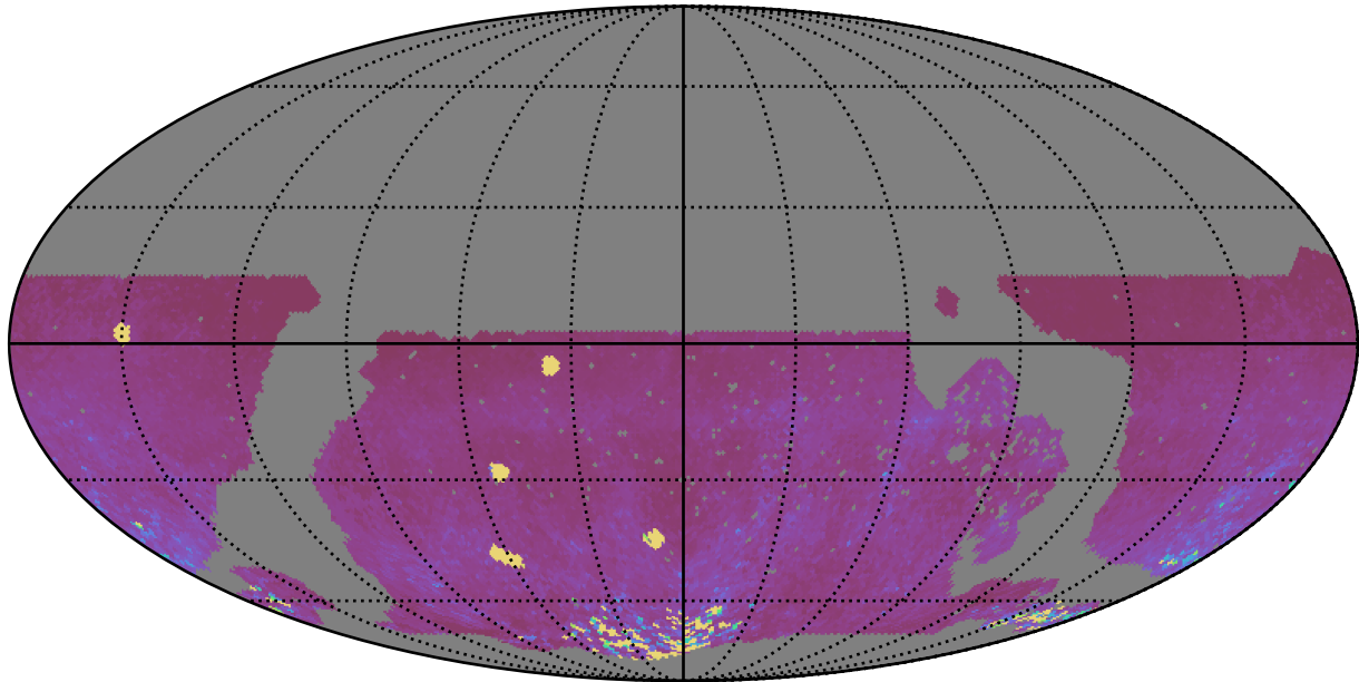
noroll_mjdp60_v3.4_10yrs WFD iz bands: 75th Percentile Intranight Timespan
