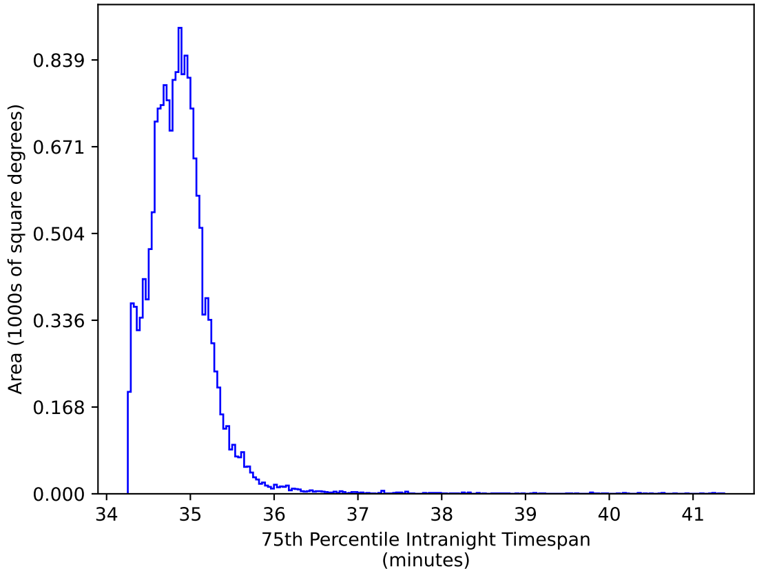
noroll_mjdp60_v3.4_10yrs WFD iz bands: 75th Percentile Intranight Timespan
