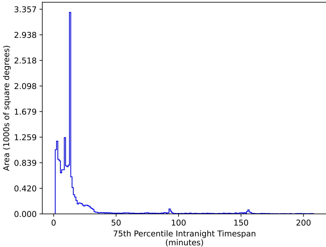
noroll_mjdp60_v3.4_10yrs WFD i band: 75th Percentile Intranight Timespan
