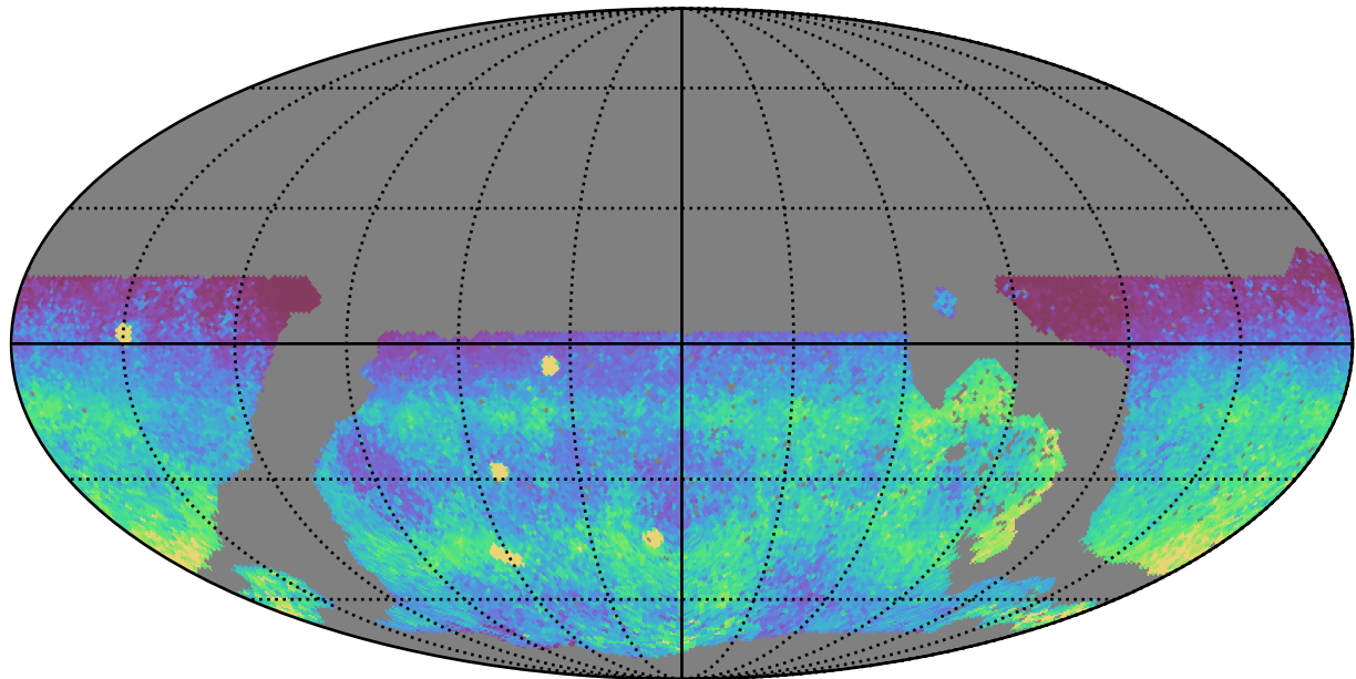
noroll_mjdp60_v3.4_10yrs WFD all bands: 75th Percentile Intranight Timespan
