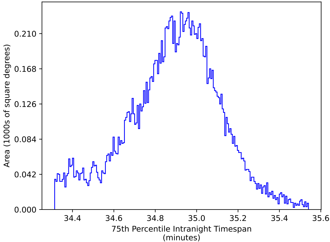
noroll_mjdp60_v3.4_10yrs WFD all bands: 75th Percentile Intranight Timespan
