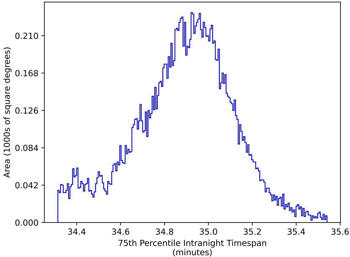
noroll_mjdp60_v3.4_10yrs WFD: 75th Percentile Intranight Timespan
