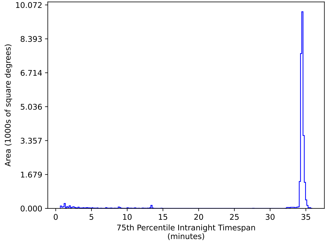
noroll_mjdp60_v3.4_10yrs All sky zy bands: 75th Percentile Intranight Timespan
