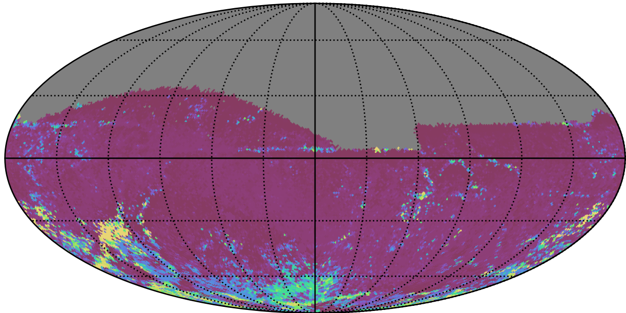
noroll_mjdp60_v3.4_10yrs All sky z band: 75th Percentile Intranight Timespan
