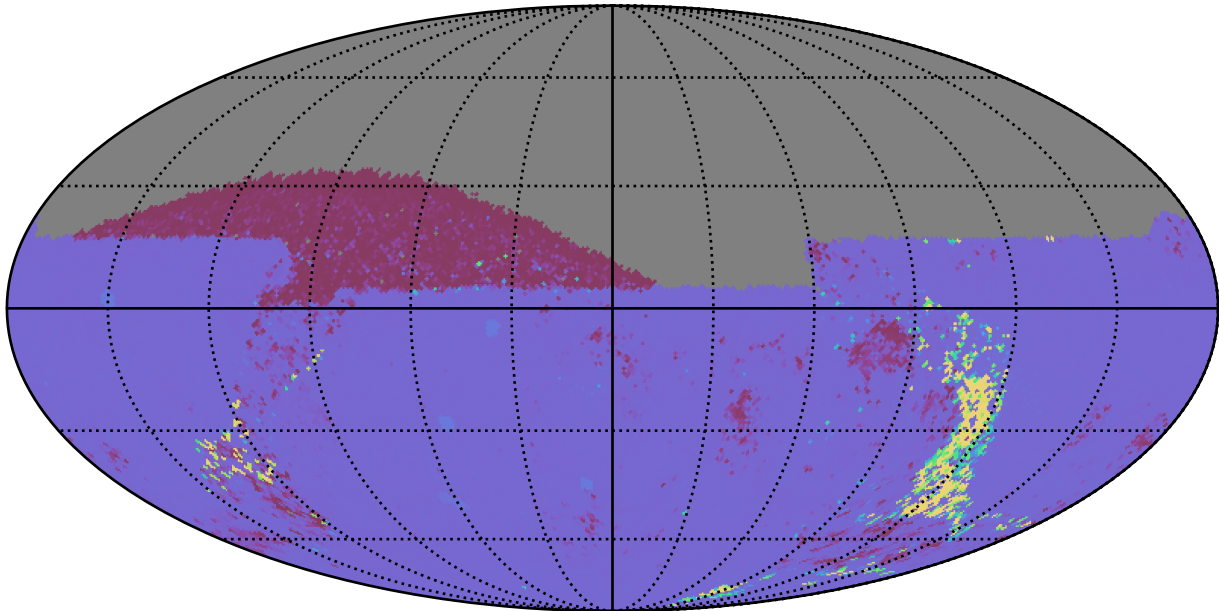
noroll_mjdp60_v3.4_10yrs All sky ug bands: 75th Percentile Intranight Timespan
