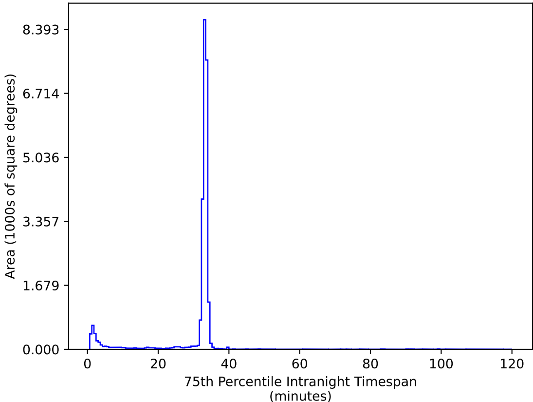
noroll_mjdp60_v3.4_10yrs All sky ug bands: 75th Percentile Intranight Timespan
