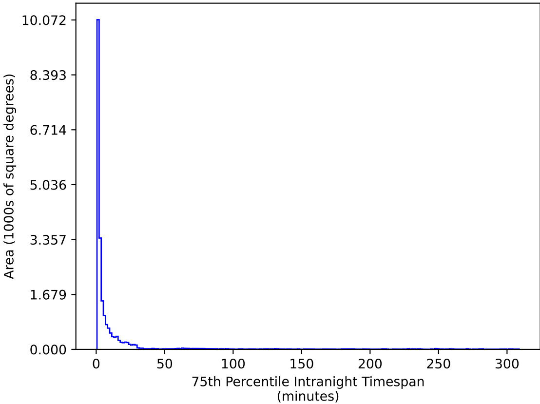
noroll_mjdp60_v3.4_10yrs All sky u band: 75th Percentile Intranight Timespan
