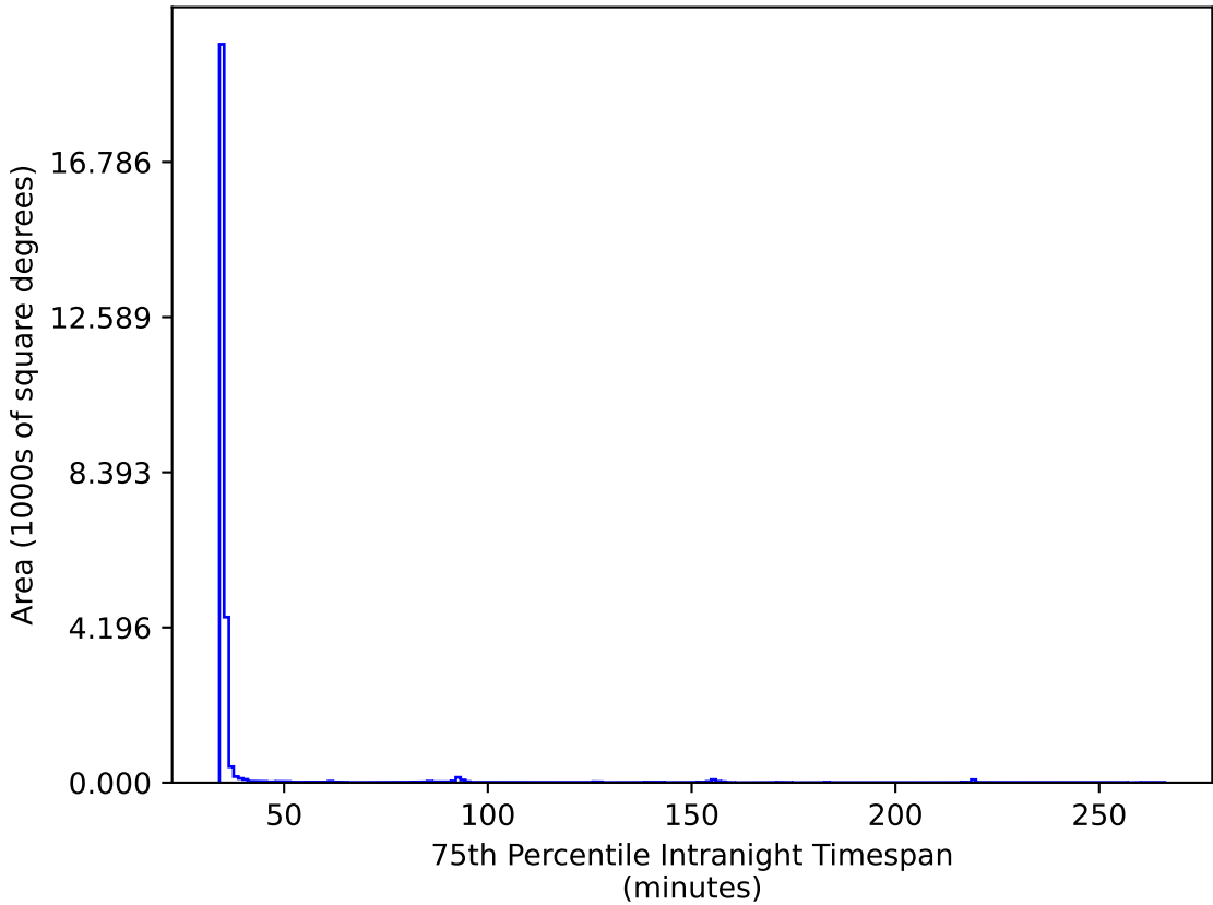
noroll_mjdp60_v3.4_10yrs All sky ri bands: 75th Percentile Intranight Timespan
