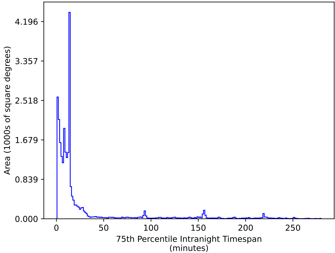
noroll_mjdp60_v3.4_10yrs All sky i band: 75th Percentile Intranight Timespan
