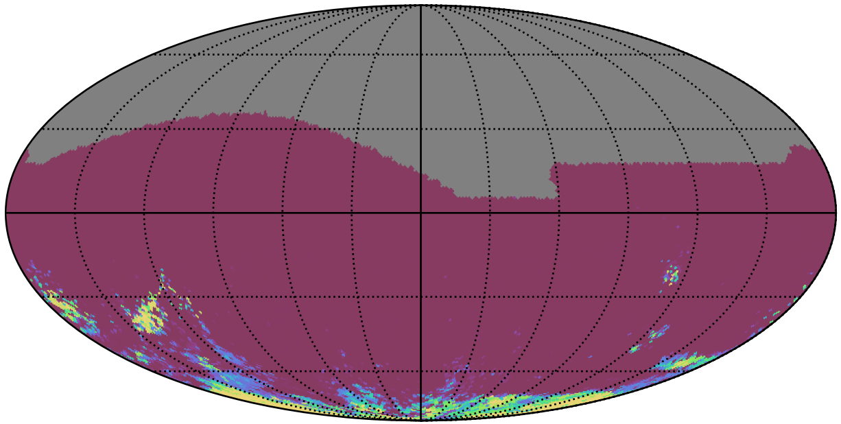
noroll_mjdp60_v3.4_10yrs All sky gr bands: 75th Percentile Intranight Timespan
