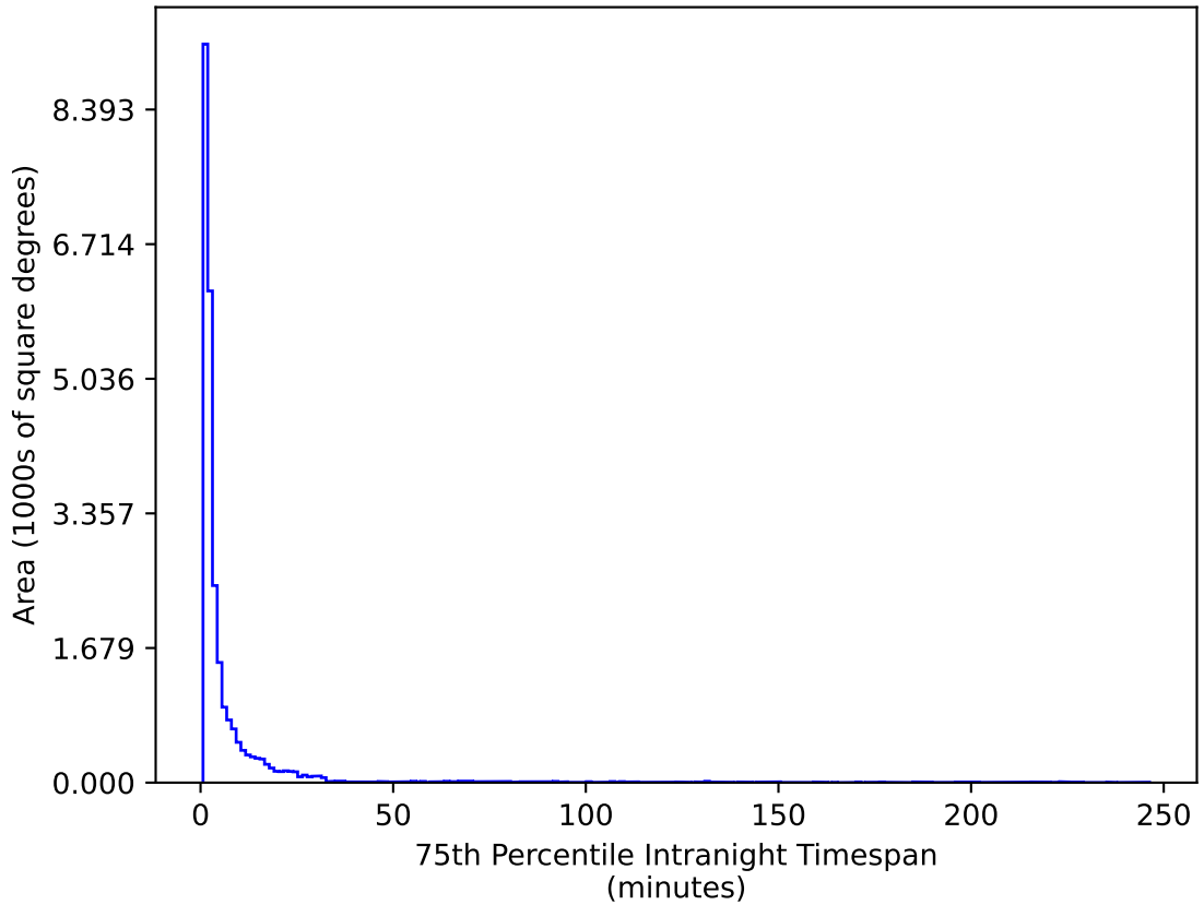
noroll_mjdp60_v3.4_10yrs All sky g band: 75th Percentile Intranight Timespan
