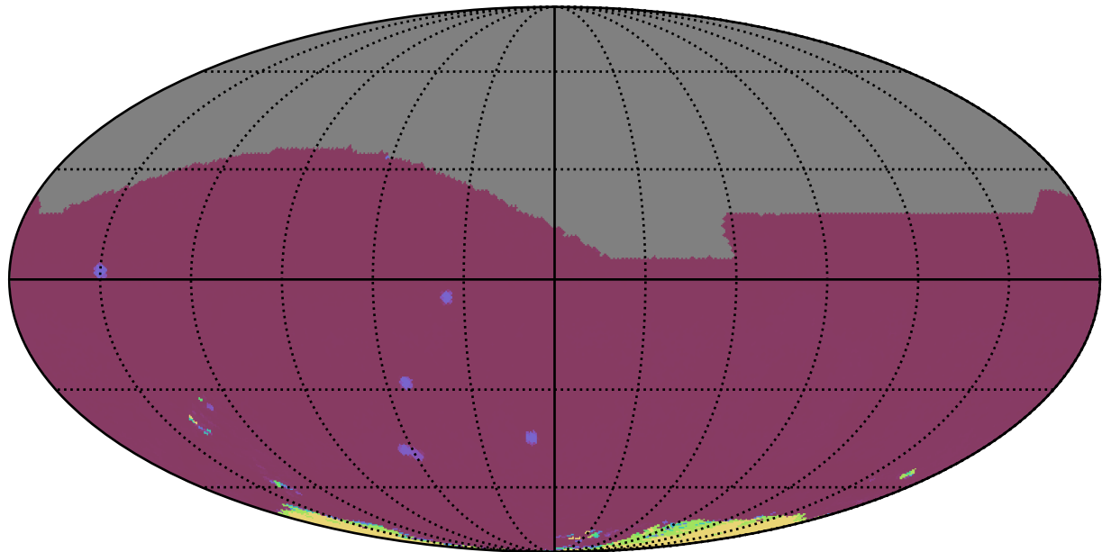
noroll_mjdp60_v3.4_10yrs All sky all bands: 75th Percentile Intranight Timespan
