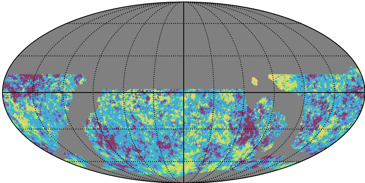
noroll_mjdp60_v3.4_10yrs WFD z band: 20thPercentile Inter-Night Gap
